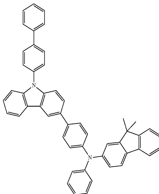
HT4
