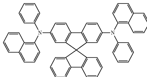
Spiro-NPB
