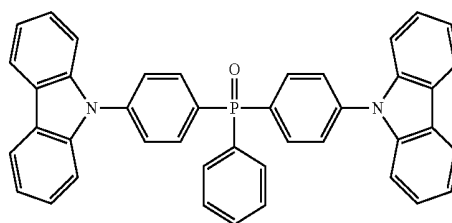
BCPO
