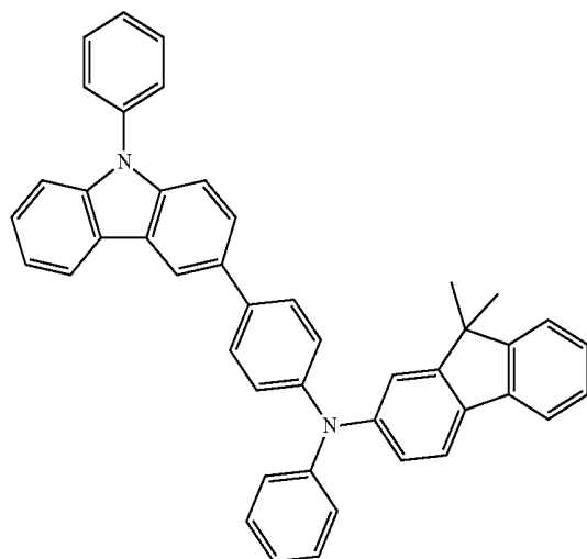
HT1
