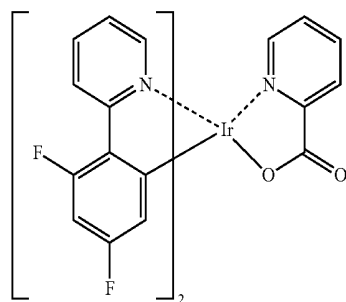
Flrpic
