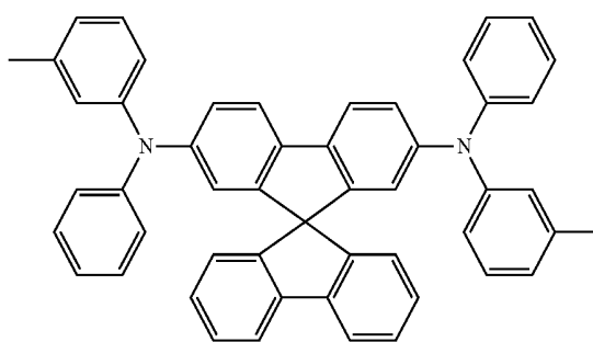
Spiro-TPD
