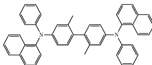
methylated NPB
