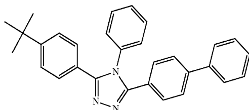
TAZ
