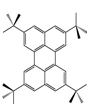
TBPe
