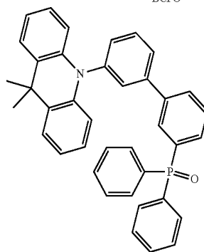
BCPO
