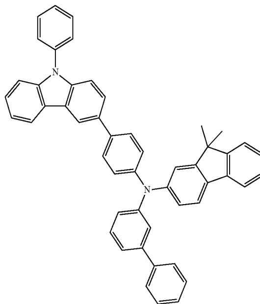
HT4
