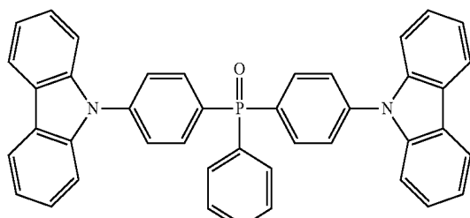
BCPO
